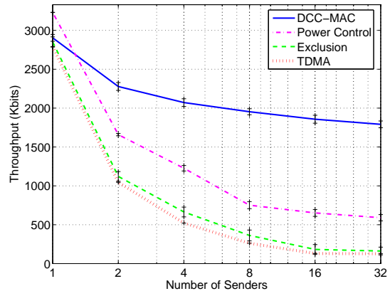
(b) Near-far scenario with sender-receiver distance of 20\text{m} and receiver-interferer distance of 1\text{m} .
