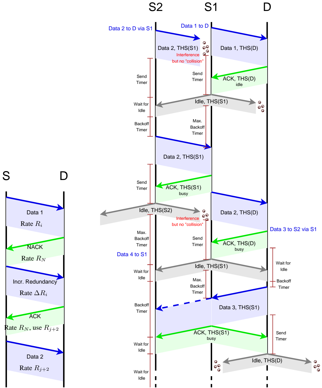
(a) Dynamic Channel Coding example: The first transmission attempt fails and additional data has to be transmitted so that the packet can be decoded. The rate to be used for subsequent packets is adjusted accordingly.
