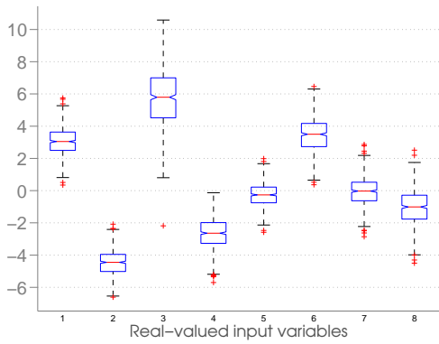
(a) Boxplot of real-valued X . Data is not centered and therefore we normalize it.
